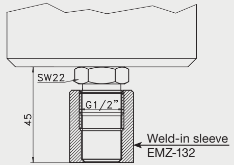
Dimensioned Drawing nozzle ITM-3 / FF
